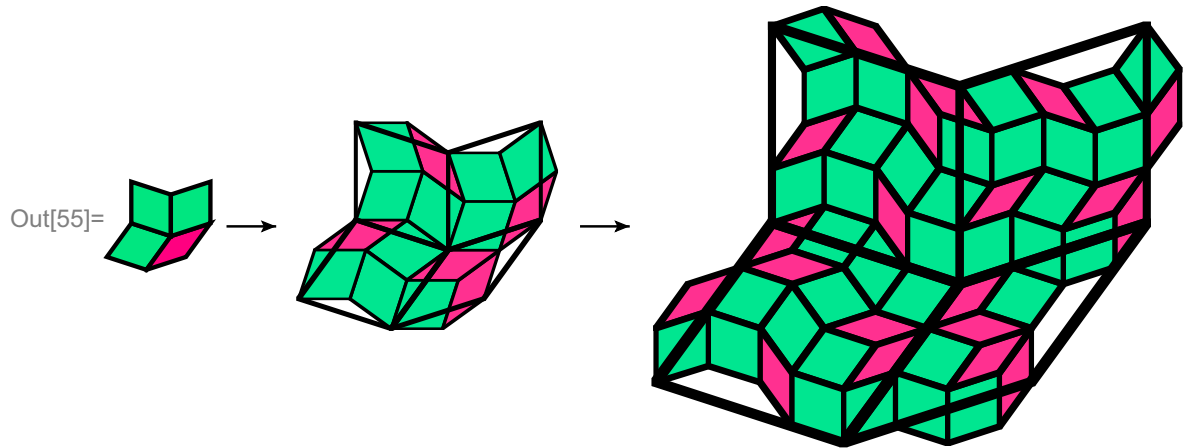
Fig. 15. How to iterate the binary substitution.
