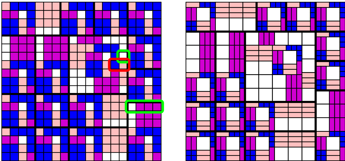
Fig. 31. Three iterates of the tile of type 1, with a loss of FLC on the right.
