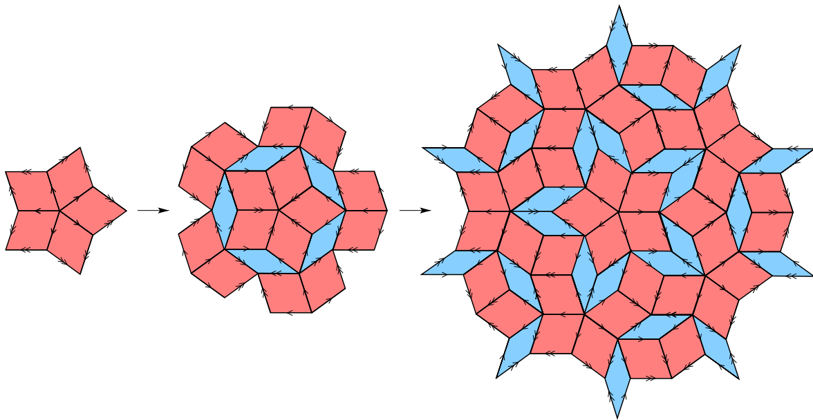
Fig. 12. A few iterations of the Penrose inflation.
