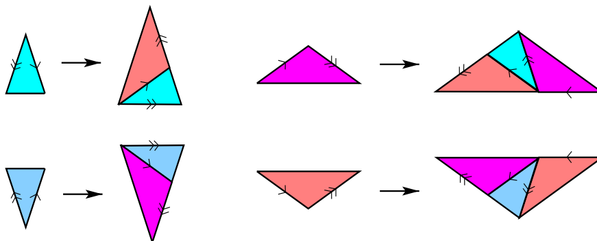
Fig. 13. The triangles version of the inflate-and-subdivide rule.
