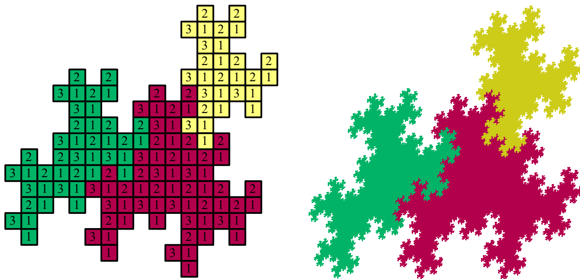
Fig. 29. A comparison of an iterate with the limiting self-similar tiles.
