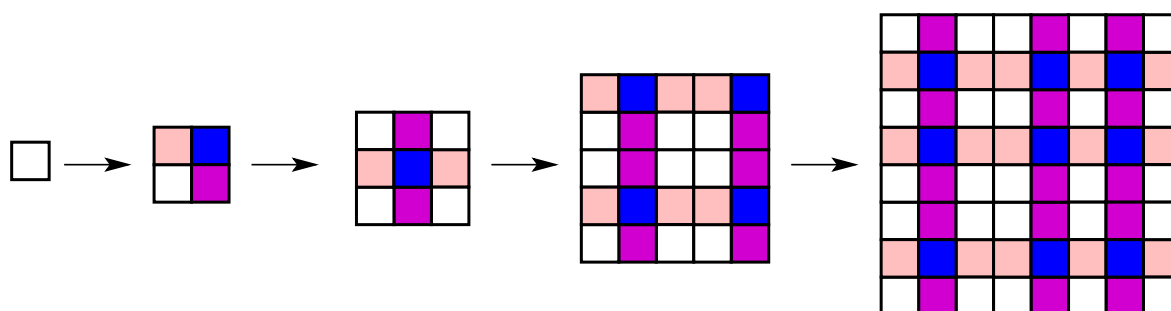
Fig. 4. A few iterations of the Fibonacci direct product substitution.
