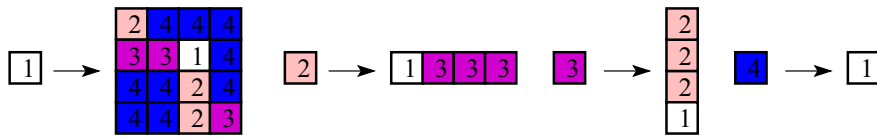
Fig. 24. A non-Pisot direct product variation substitution.
