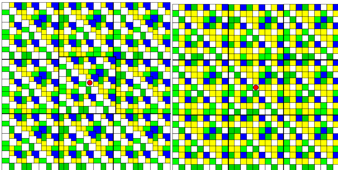
Fig. 39. Comparing three iterations of the white square.
