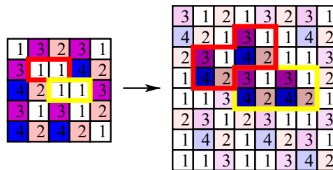
Fig. 20. The substitution of an adjacent pair of tiles depends on its context.
