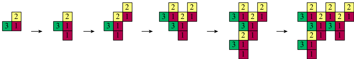
Fig. 23. A few iterates of the Rauzy two-dimensional substitution.
