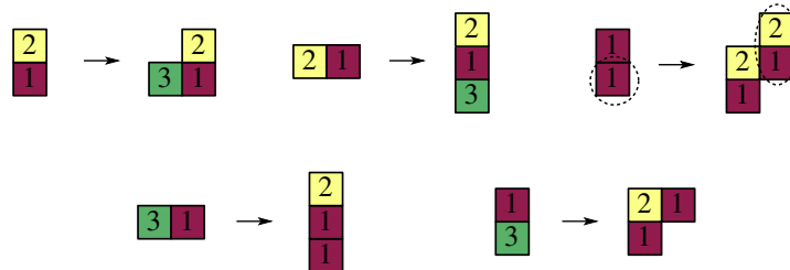
Fig. 22. How to substitute important adjacencies for the Rauzy substitution.
