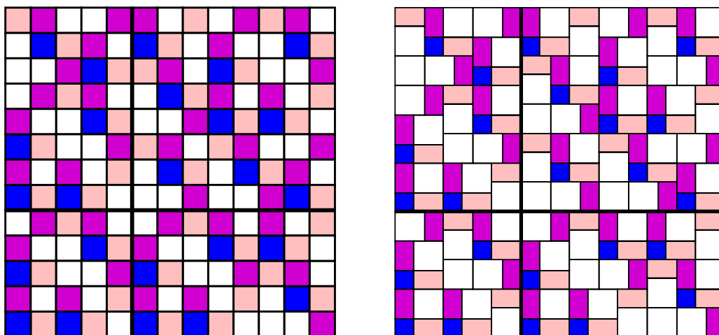
Fig. 28. Comparing the DPV with the SST of Example 15.
