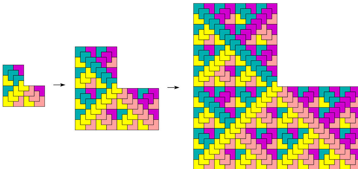
Fig. 6. Level-2, level-3, and level-4 tiles.
