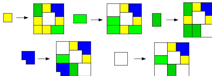
Fig. 37. The Chacon primitive substitution.
