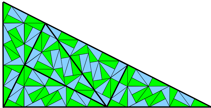
Fig. 8. A level-3 tile for the pinwheel inflation.
