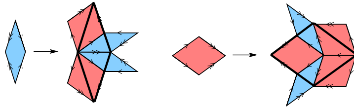
Fig. 11. The “Penrose inflation”: an imperfect substitution rule.
