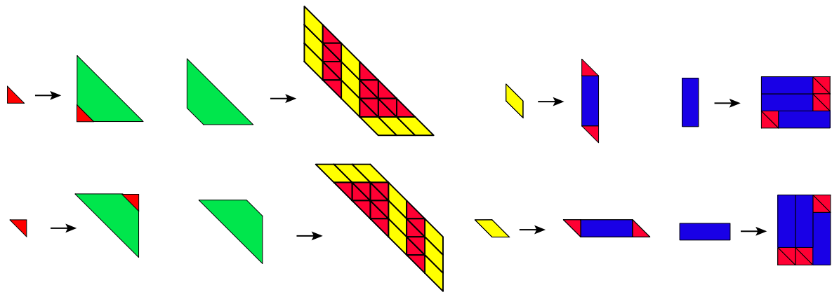
Fig. 25. A substitution similar to one in [12].
