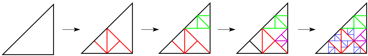
Fig. 10. A special case of the generalized pinwheel tilings: \alpha = \pi/4 .
