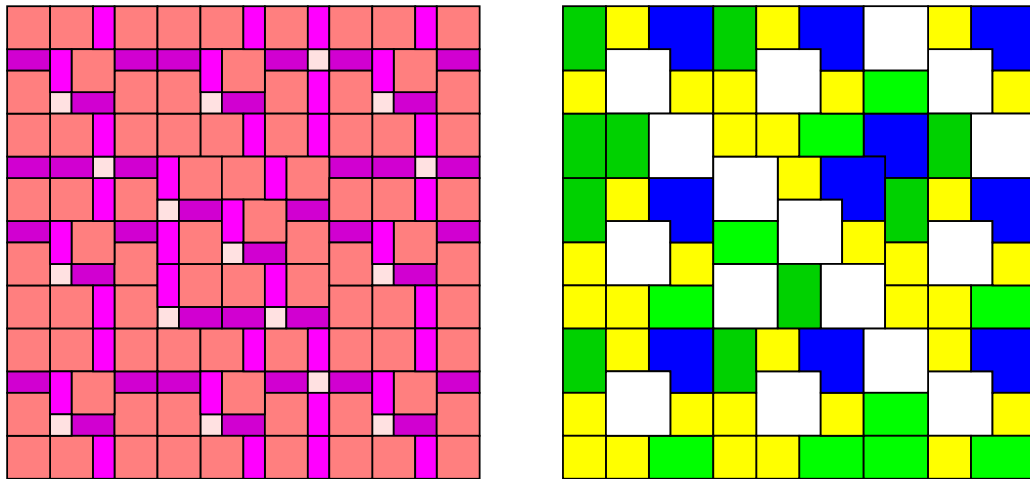
Fig. 36. Chacon level-two tiles, non-primitive and primitive versions.
