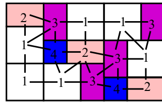
Fig. 17. Dually situated tiling and graph.
