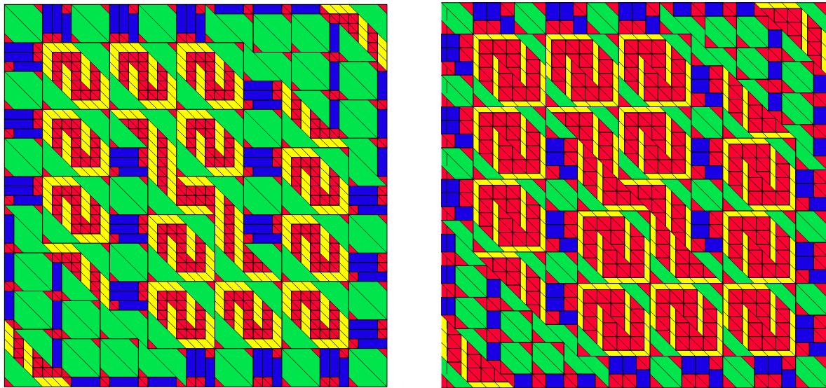
Fig. 32. Four iterations of a square formed by two red triangles. Fault lines occur in three directions in the tiling on the right.
