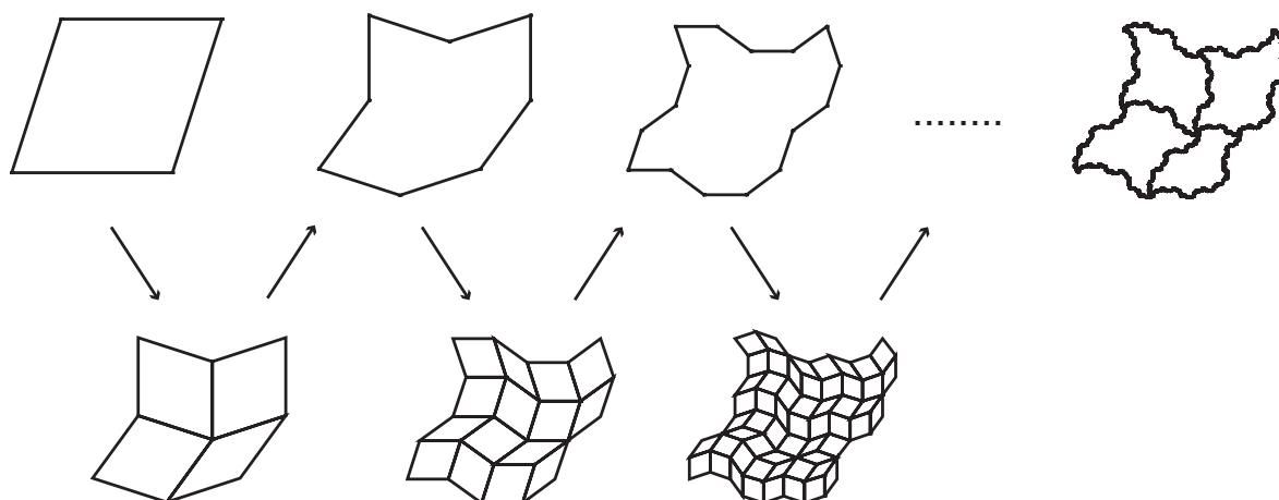
Fig. 16. Obtaining fractal binary tiles.
