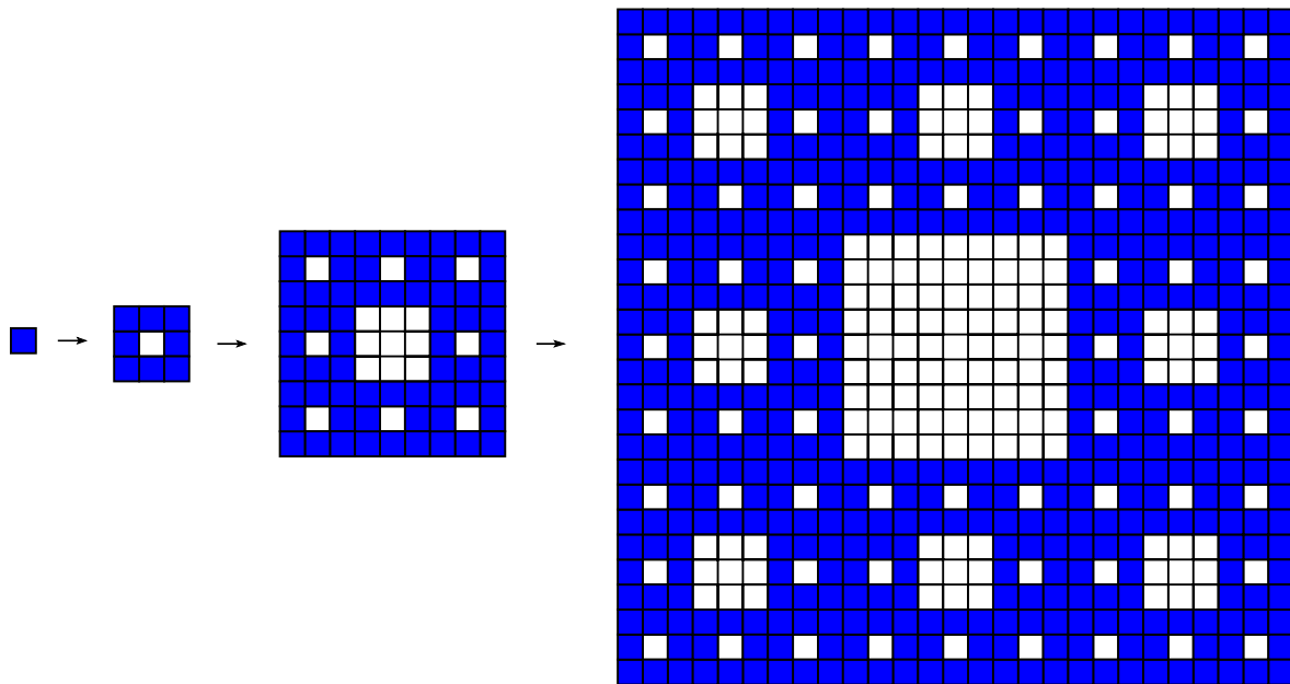
Fig. 2. Level-0, level-1, level-2, and level-3 tiles.
