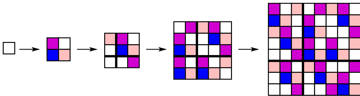
Fig. 19. Iterating of the Fibonacci DPV on the tile of type 1.
