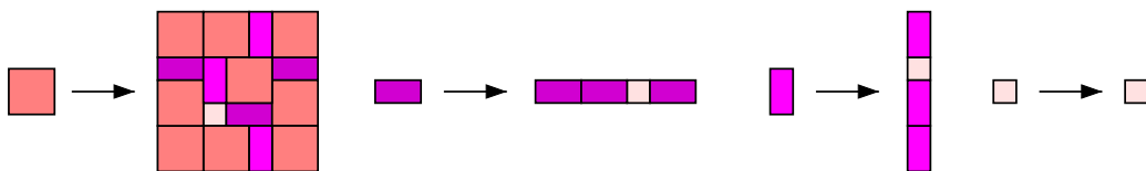
Fig. 34. The Chacon cut-and-stack construction found in [34].
