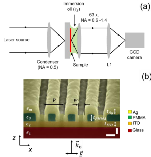
Fig. 1. (a) Schematic LRM experimental setup used for the acquisition of images. (b) SEM image (false color) of the sample structure, where w is the width of the grating and p the pitch; t_{\text{Ag}} , t_{\text{PMMA}} and t_{\text{ITO}} are the thicknesses of the Ag, PMMA and ITO films, respectively. The arrows represent the wave vector \vec{k}_o and electric field of the excitation field \vec{E} . The scale bars represent 200 nm in the vertical and horizontal directions and the color chart shows the materials used in the sample.
