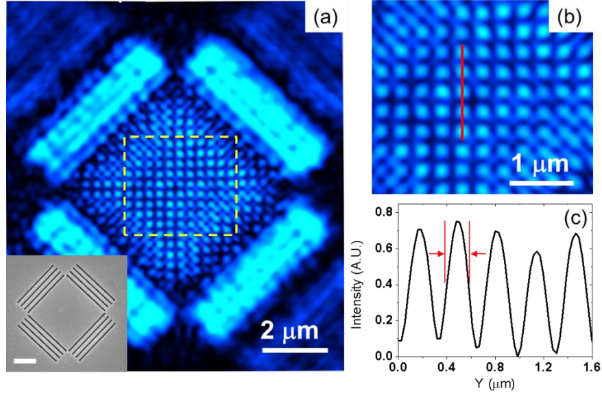
Fig. 4. (a) Optical image taken with the proposed LRM of a plasmonic cavity composed of four perpendicular gratings with width 150 nm and pitch 440 nm. The excitation wavelength was 473 nm. The inset is an SEM image, with a 2 μm the scale bar. (b) Detailed view inside the dashed rectangle in (a). (c) Intensity profile measured along the red line in (b), showing the FWHM.
