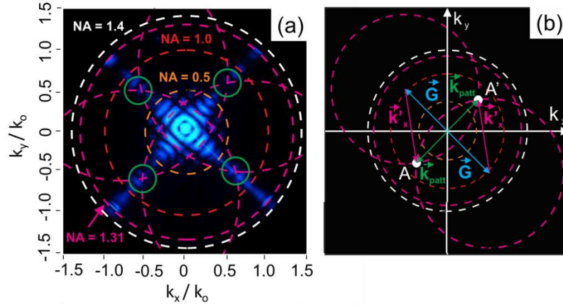
Fig. 5. (a) Fourier space image of the plasmonic cavity presented in Fig. 4(a). The orange, red, purple and white circles are associated with NA = 0.5, 1.0, 1.31 and = 1.4, respectively, as indicated. The purple dashed lines are related to k_x' displaced by \vec{G} . (b) k-space analysis of experimental Fourier space image in (a). The scale has been changed in order to allow the observation of the complete scheme, but the proportion is the same. The vectors \vec{G} , \vec{k}_x and \vec{k}_{pat} are the wavevectors of the grating, SP and the observed pattern respectively. The distance between points A and A' shows the wavenumber of the observed pattern.
