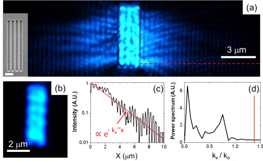
Fig. 2. LRM image acquired by the proposed configuration using NA = 1.4 (a) and far field image using NA = 0.6 (b). The excitation wavelength was 473 nm. The inset to (a) is an SEM image of the grating with w = 150 nm and p = 440 nm. Inset scale bar: 1 μm. (c) Intensity registered in the red line in (a) using logarithmic scale. The red arrow shows an exponential decay shape. (d) Power spectrum calculated from the intensity profile shown in (c). The red line shows the maximum used NA.
