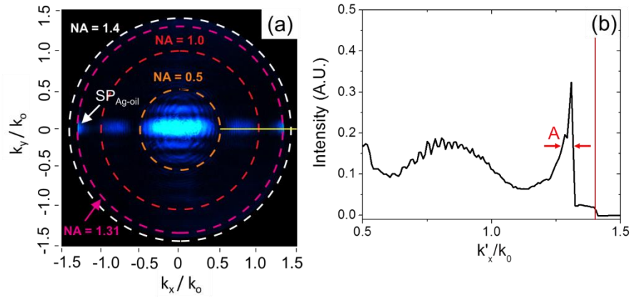
Fig. 3. (a) Fourier space image normalized to the excitation wavenumber of the leaked field in Fig. 2(a). The white circle represents NA = 1.4 , while red and orange circles are NA = 1 and 0.5 , respectively. (b) Transversal cut made in the yellow line in (a). The arrows represent the distance A measured at FWHM.
