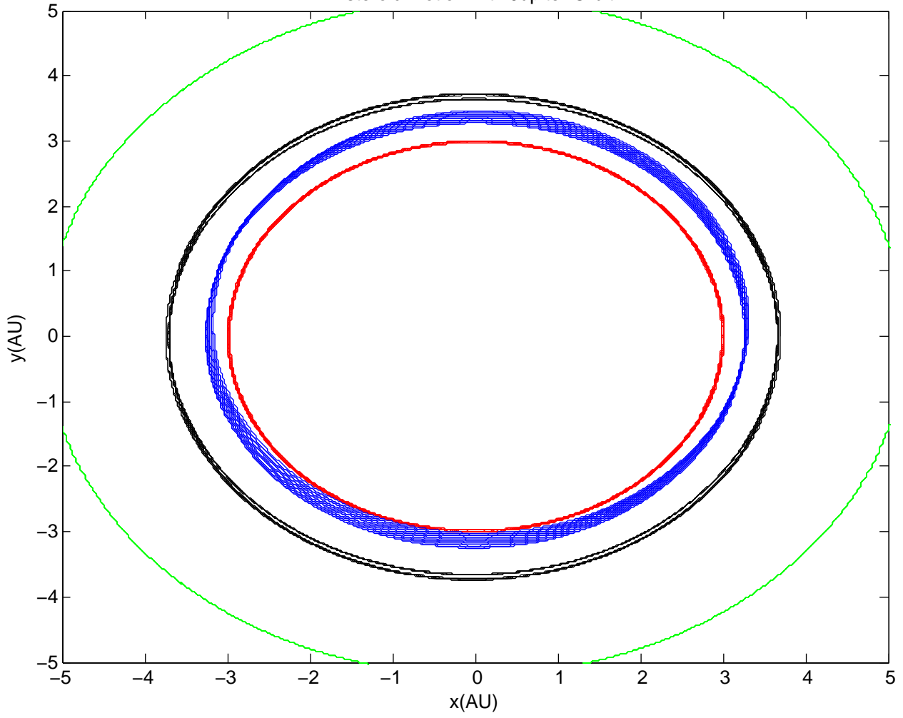
Asteroid Motion with Jupiter Orbit
